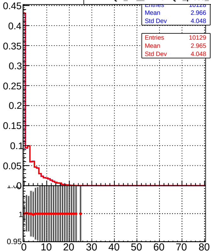
Legend: DQM_TT_mkFit-DQM_pless_orig (grey bars) DQM_TT_mkFit-DQM_pless_mod (red line with dots)
