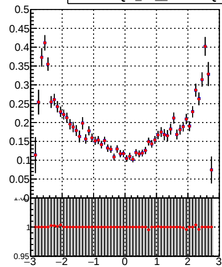
■ — ● DQM_TT_mkFit-DQM_pless_orig — ● DQM_TT_mkFit-DQM_pless_mod
