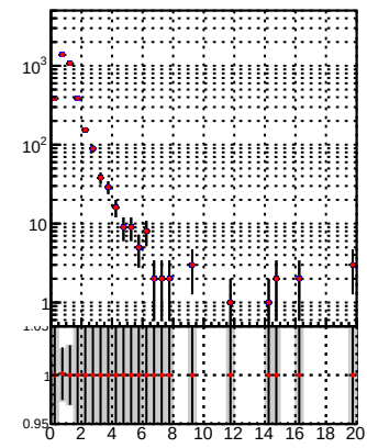
N of reco track vs. \chi^2 for DQM TT and mkFit-DQM_pless_mod
