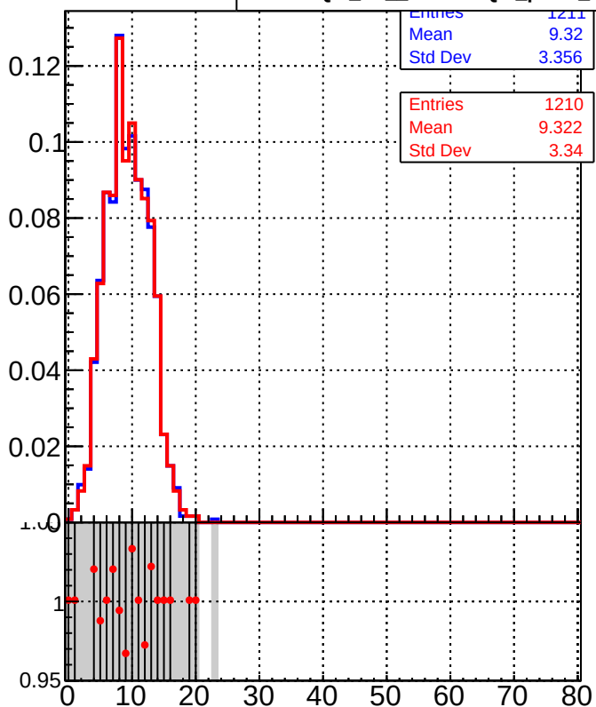
— DQM_TT_mkFit-DQM_pless_orig — DQM_TT_mkFit-DQM_pless_mod
