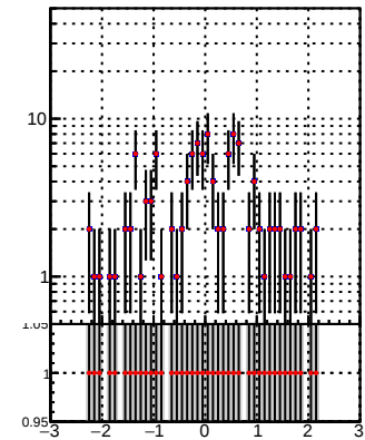
N of reco track vs \eta pT [GeV] —•— DQM TT mkFit-DQM pless_orig —•— DQM TT mkFit-DQM pless_mod
