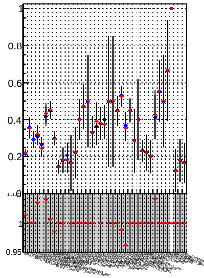
Fake rate vs. —●— DQM_TT_mkFit-DQM_pless_orig —●— DQM_TT_mkFit-DQM_pless_mod
