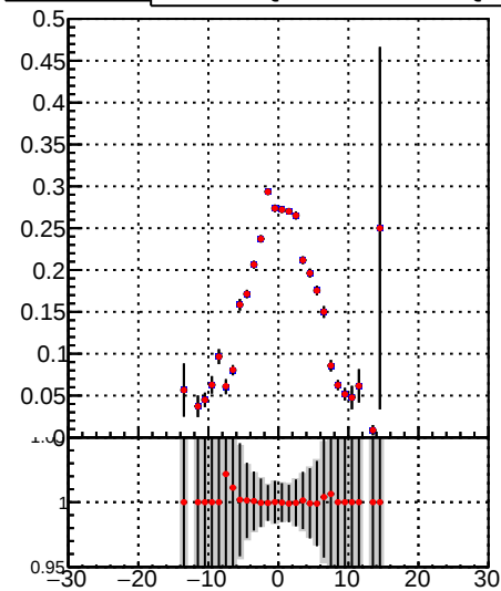
—•— DQM_TT_mkFit-DQM_pless_orig —•— DQM_TT_mkFit-DQM_pless_mod
