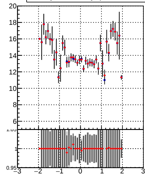
mean hit — DQM_TT_mkFit-DQM_pless_orig — DQM_TT_mkFit-DQM_pless_mod
