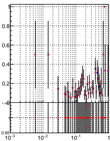
—●— DQM_TT_mkFit-DQM_pless_orig —●— DQM_TT_mkFit-DQM_pless_mod
