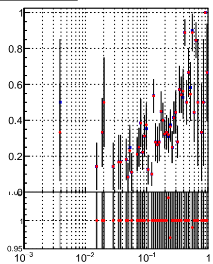
—●— DQM_TT_mkFit-DQM_pless_orig —●— DQM_TT_mkFit-DQM_pless_mod
