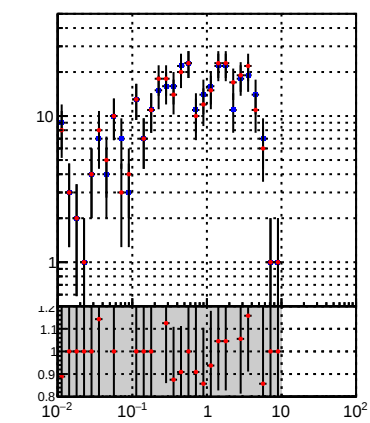
N of associated (recoToSim) loopers vs transverse ref point position
