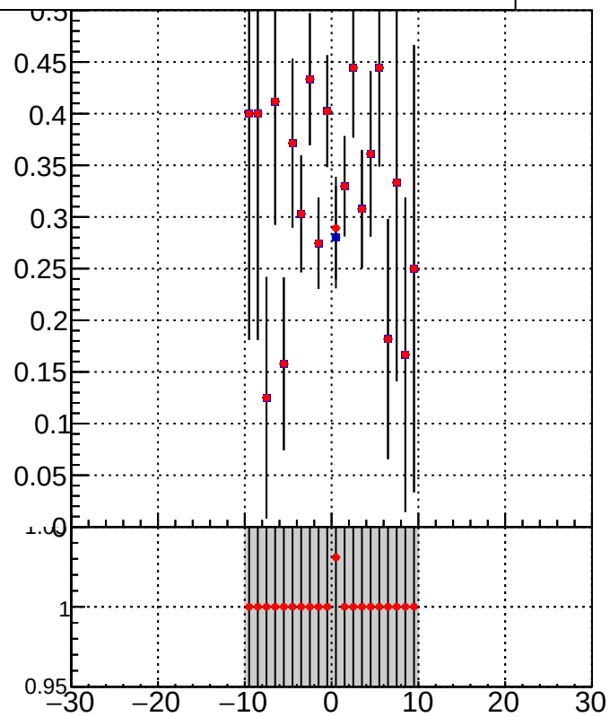
DQM_TT_mkFit-DQM_pless_orig DQM_TT_mkFit-DQM_pless_mod
