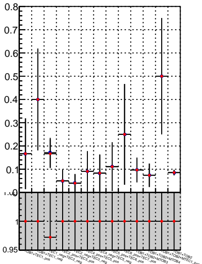
Fake rate vs. — DQM_TT_mkFit-DQM_pless_orig — DQM_TT_mkFit-DQM_pless_mod
