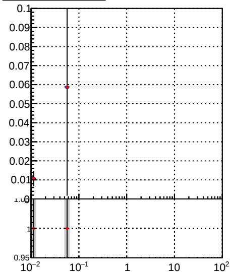
█ DQM_TT_mkFit-DQM_pless_orig █ DQM_TT_mkFit-DQM_pless_mod
