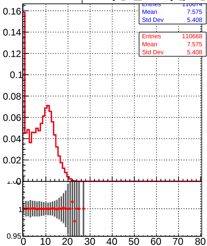
— DQM_TT_mkFit-DQM_pless_orig — DQM_TT_mkFit-DQM_pless_mod
