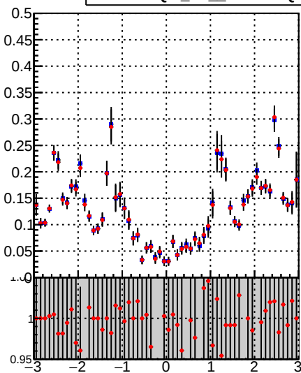
—■— DQM_TT_mkFit-DQM_pless_orig —●— DQM_TT_mkFit-DQM_pless_mod
