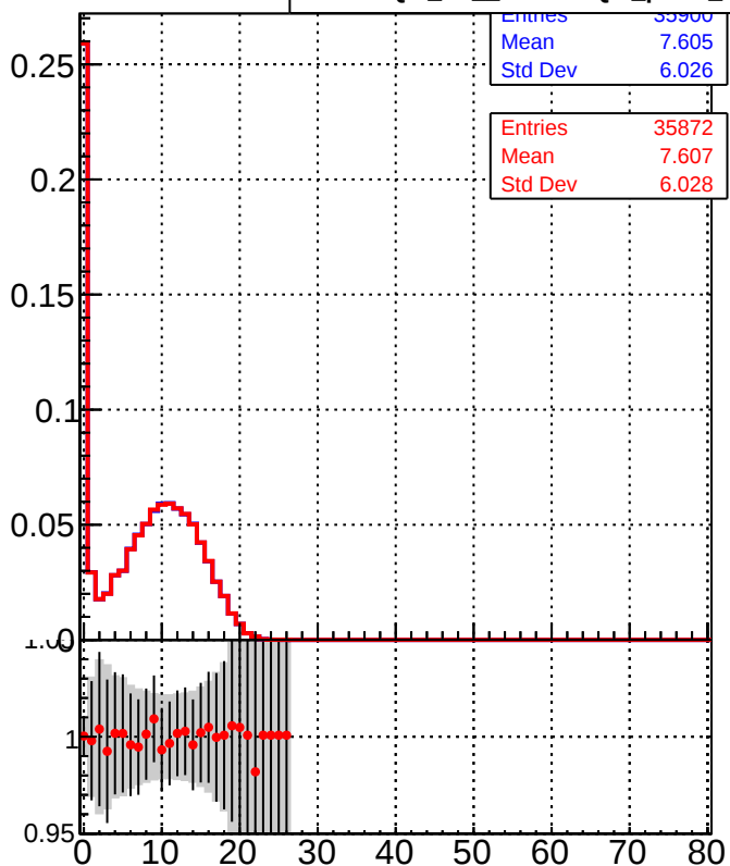
Legend: DQM_TT_mkFit-DQM_pless_orig (grey bars) DQM_TT_mkFit-DQM_pless_mod (red line)
