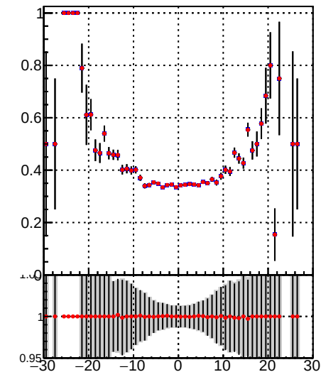
—•— DQM_TT_mkFit-DQM_pless_orig —•— DQM_TT_mkFit-DQM_pless_mod
