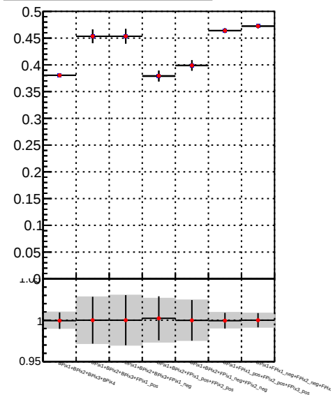
Fake rate vs. \bullet DQM TT mkFit-DQM_pless_orig \bullet DQM TT mkFit-DQM_pless_mod
