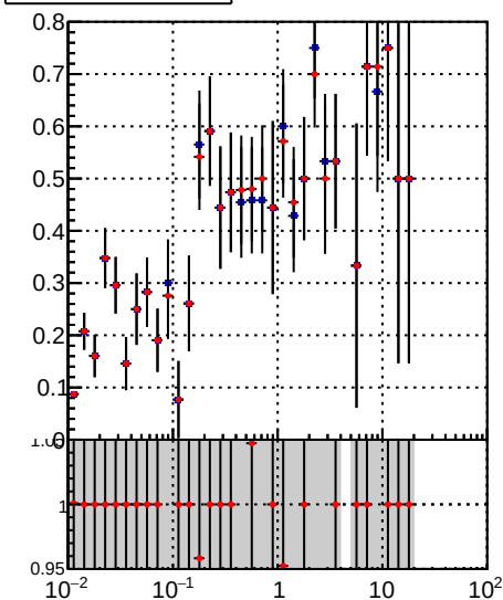
—•— DQM_TT_mkFit-DQM_pless_orig —•— DQM_TT_mkFit-DQM_pless_mod
