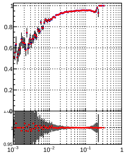
Fake rate vs DQM_TT_mkFit-DQM_pless_orig DQM_TT_mkFit-DQM_pless_mod
