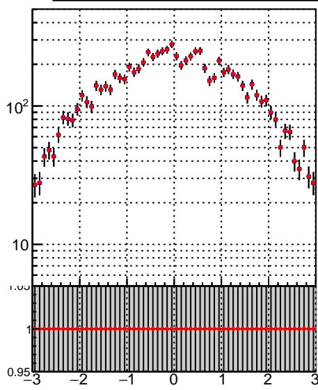
■ DQM_TT_mkFit-DQM_pless_orig ◆ DQM_TT_mkFit-DQM_pless_mod
