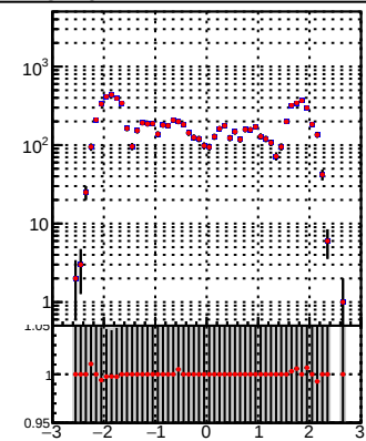
—•— DQM_TT_mkFit-DQM_pless_orig —•— DQM_TT_mkFit-DQM_pless_mod
