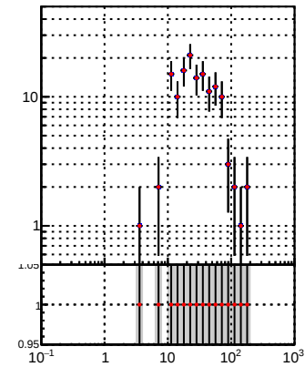
—●— DQM_TT_mkFit-DQM_pless_orig —●— DQM_TT_mkFit-DQM_pless_mod
