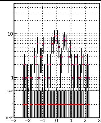
—●— DQM_TT_mkFit-DQM_pless_orig —●— DQM_TT_mkFit-DQM_pless_mod
