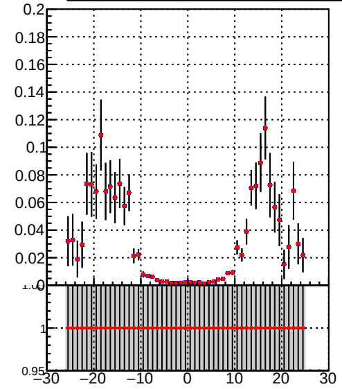
Efficiency vs. sim PV z — DQM_TT_mkFit-DQM_pless_orig — DQM_TT_mkFit-DQM_pless_mod
