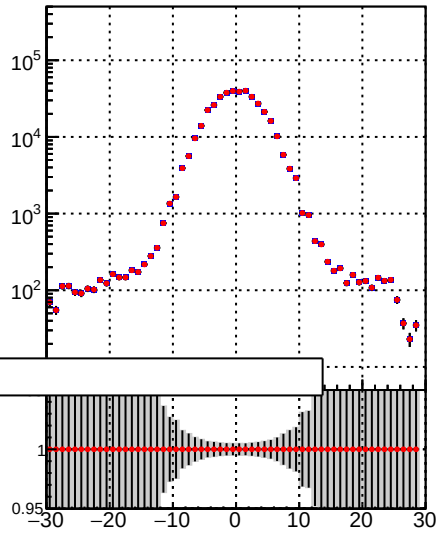
N of simulated tracks vs z vert position
