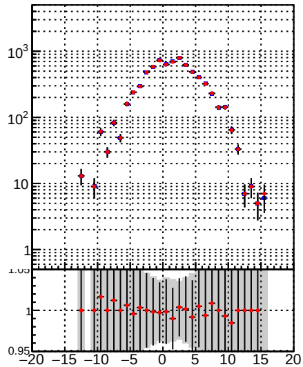
N of associated tracks (simToReco) vs. sim PV z
