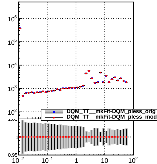
N of simulated tracks vs transverse vert position
