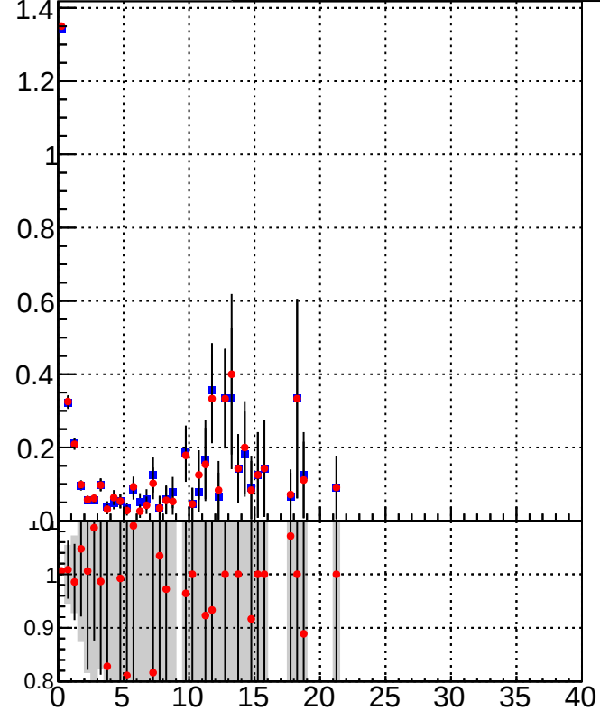
K_S^0 tracking fake rate vs p_T (Detailed View) Legend: \blacksquare DQM_TT_mkFit-DQM_pless_orig \bullet DQM_TT_mkFit-DQM_pless_mod
