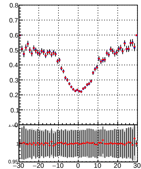
—•— DQM_TT_mkFit-DQM_pless_orig —•— DQM_TT_mkFit-DQM_pless_mod
