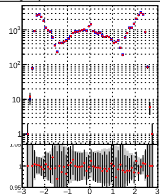
—•— DQM_TT_mkFit-DQM_pless_orig —•— DQM_TT_mkFit-DQM_pless_mod
