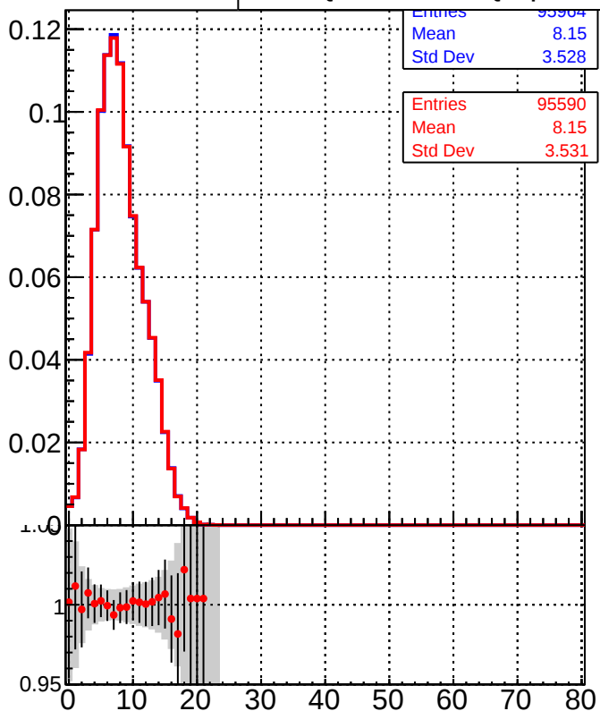
Legend for the bottom row plots: DQM_TT_mkFit-DQM_pless_orig (Blue line with markers) DQM_TT_mkFit-DQM_pless_mod (Red line with markers)
