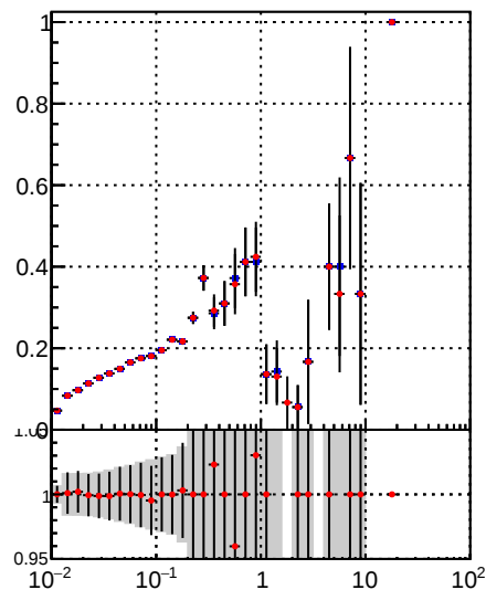
—•— DQM_TT_mkFit-DQM_pless_orig —•— DQM_TT_mkFit-DQM_pless_mod
