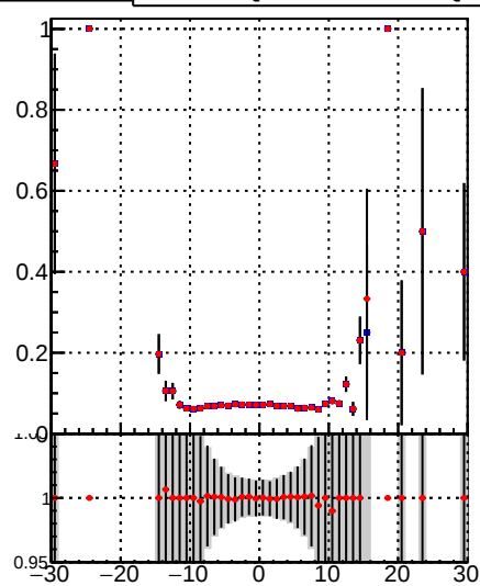
—•— DQM_TT_mkFit-DQM_pless_orig —•— DQM_TT_mkFit-DQM_pless_mod
