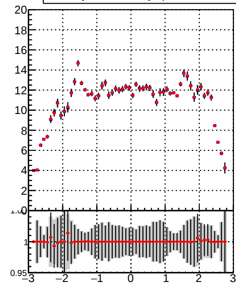
— DQM_TT_mkFit-DQM_pless_orig — DQM_TT_mkFit-DQM_pless_mod
