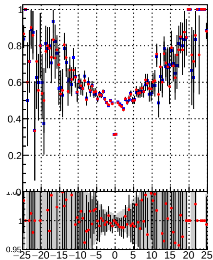
Fake rate vs xy
