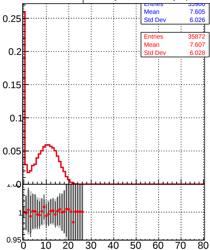
Legend: DQM_TT_mkFit-DQM_pless_orig (grey bars) DQM_TT_mkFit-DQM_pless_mod (red line with markers)
