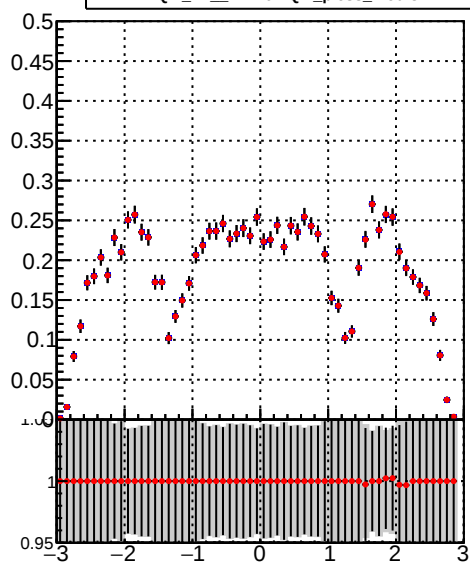
DQM_TT_mkFit-DQM_pless_orig DQM_TT_mkFit-DQM_pless_modi3
