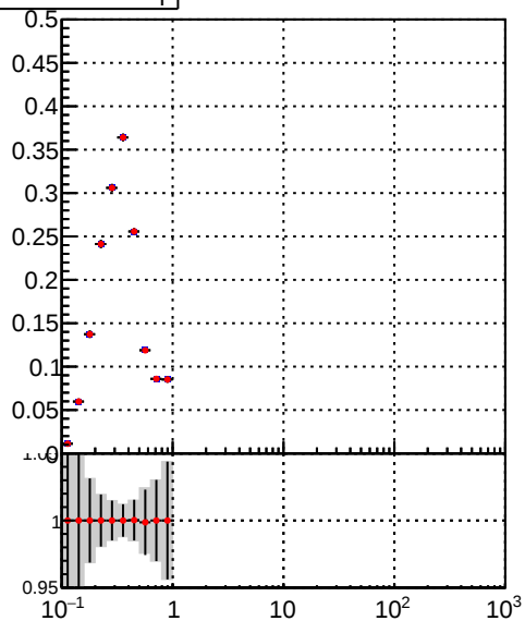
DQM_TT_mkFit-DQM_pless_orig DQM_TT_mkFit-DQM_pless_modi3
