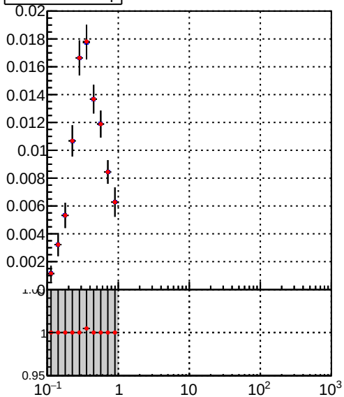
Legend: — DQM_TT_mkFit-DQM_pless_orig — DQM_TT_mkFit-DQM_pless_modi3
