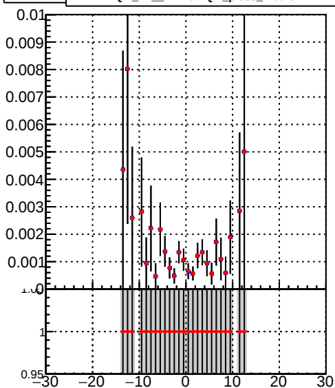
Efficiend —●— DQM_TT_mkFit-DQM_pless_modi3
