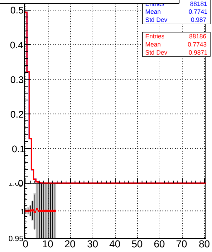
Legend: DQM_TT_mkFit-DQM_pless_orig (grey histogram), DQM_TT_mkFit-DQM_pless_modi3 (red line with markers)
