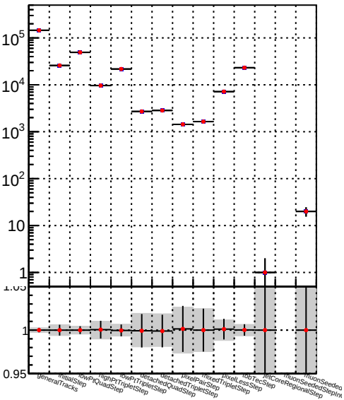
Number —●— DQM_TT_mkFit-DQM_pless_modi3
