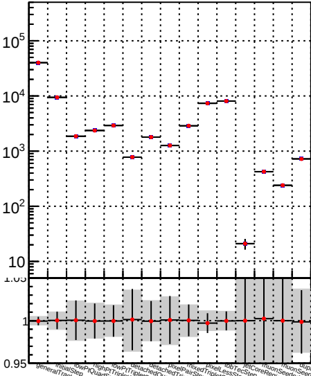
Number —●— DQM_TT_mkFit-DQM_pless_modi3
