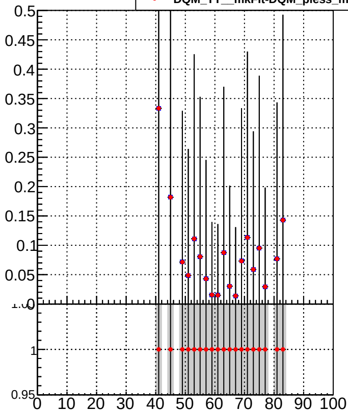
■ DQM_TT_mkFit-DQM_pless_orig ● DQM_TT_mkFit-DQM_pless_modi3
