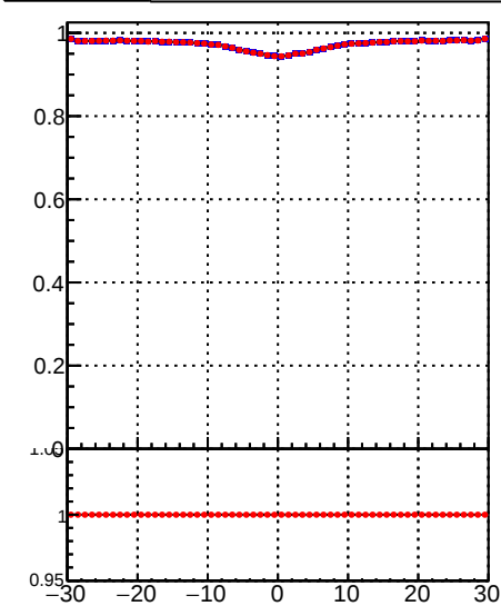
—•— DQM_TT_mkFit-DQM_pless_orig —•— DQM_TT_mkFit-DQM_pless_modi3
