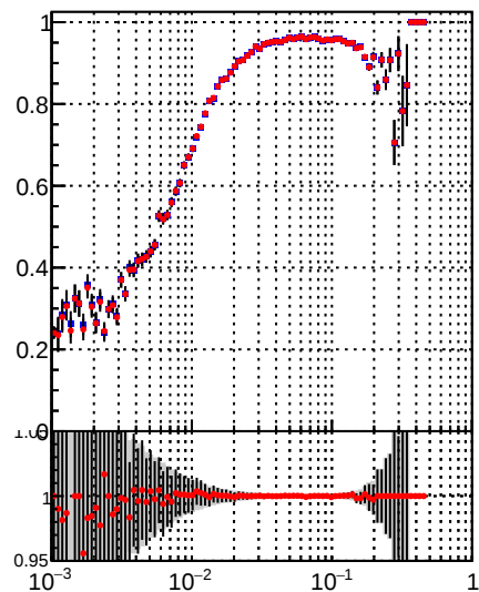
Fake rate vs \sqrt{s} Legend: DQM_TT_mkFit-DQM_pless_orig (black line with error bars) DQM_TT_mkFit-DQM_pless_modi3 (red line with error bars)
