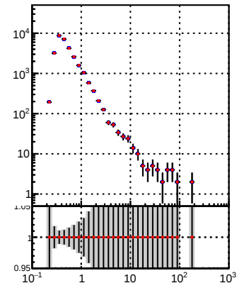
—●— DQM_TT_mkFit-DQM_pless_orig —●— DQM_TT_mkFit-DQM_pless_modi3
