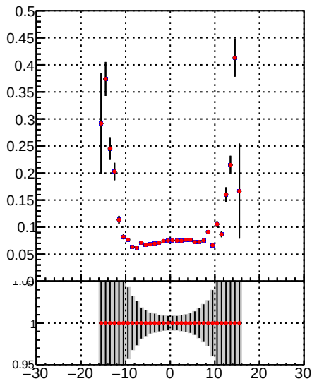
Fake rate vs d Legend: - DQM TT mkFit-DQM_pless_orig (blue line with dots) - DQM TT mkFit-DQM_pless_modi3 (red line with dots)
