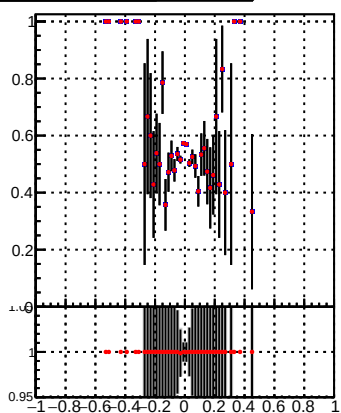
DQM_TT_mkFit-DQM_pless_modi3
