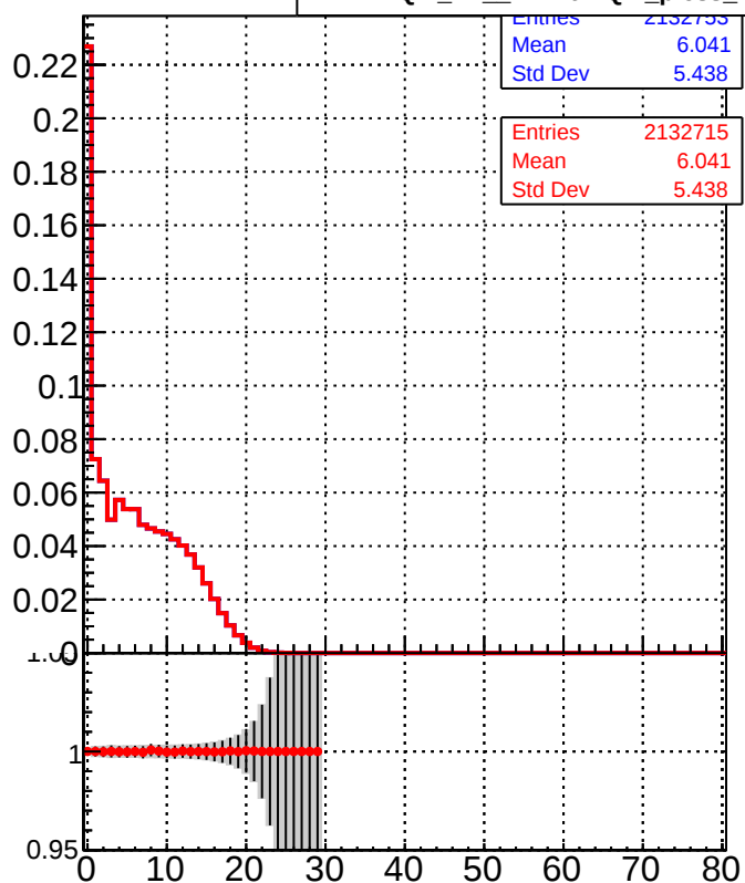
DQM_TT_mkFit-DQM_pless_orig DQM_TT_mkFit-DQM_pless_modi3
