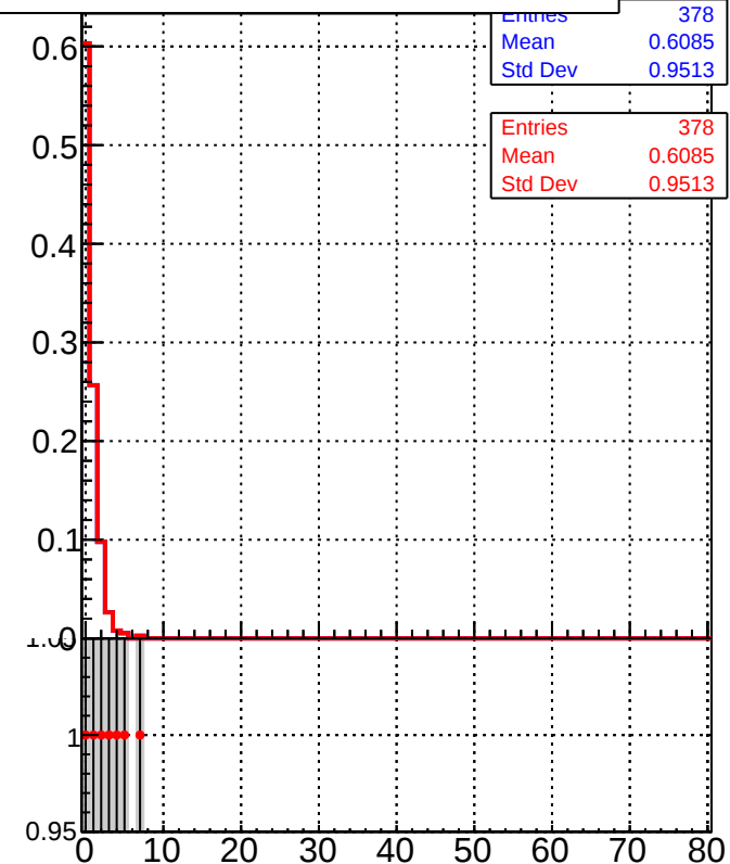
Legend: DQM_TT_mkFit-DQM_pless_orig (blue line with markers) DQM_TT_mkFit-DQM_pless_modi3 (red line with markers)
