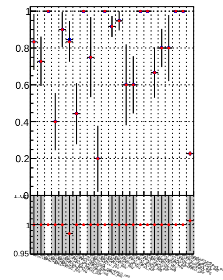
Fake rate vs. — DQM_TT_mkFit-DQM_pless_orig — DQM_TT_mkFit-DQM_pless_modi3
