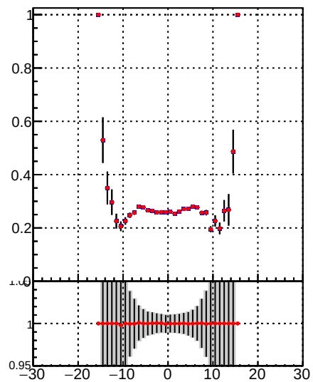
Fake rate vs d —•— DQM TT mkFit-DQM_pless_orig —•— DQM TT mkFit-DQM_pless_modi3
