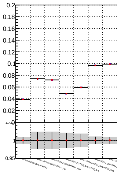
Fake rate vs. — DQM TT mkFit-DQM_pless_orig — DQM TT mkFit-DQM_pless_modi3
